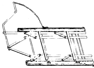
SKETCH OF HEADGATE
